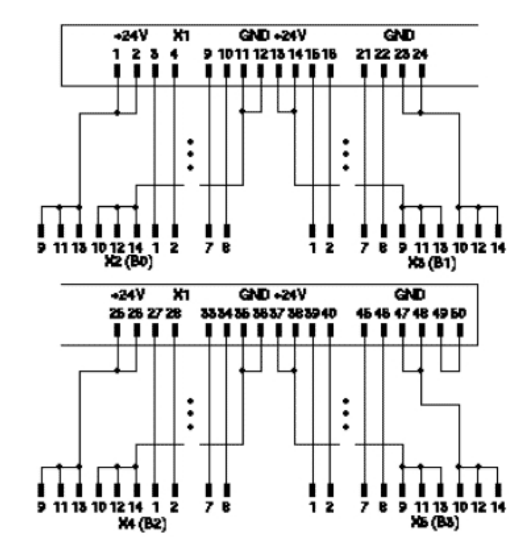
Circuit diagram
