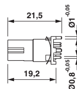
Dimensioned drawing
