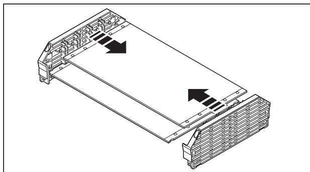
Figure 25 PCBs, horizontal
