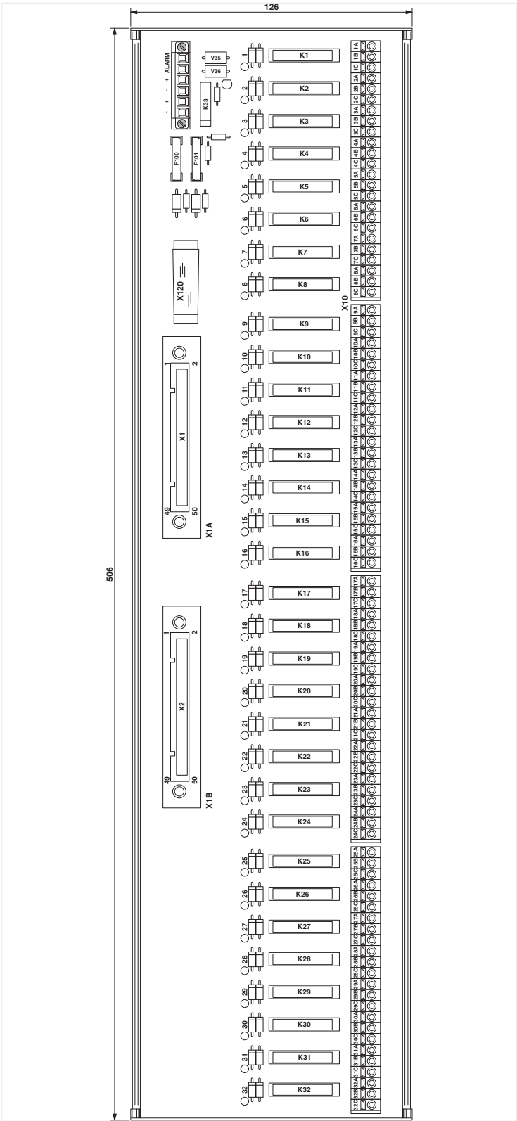
Dimensional drawing
