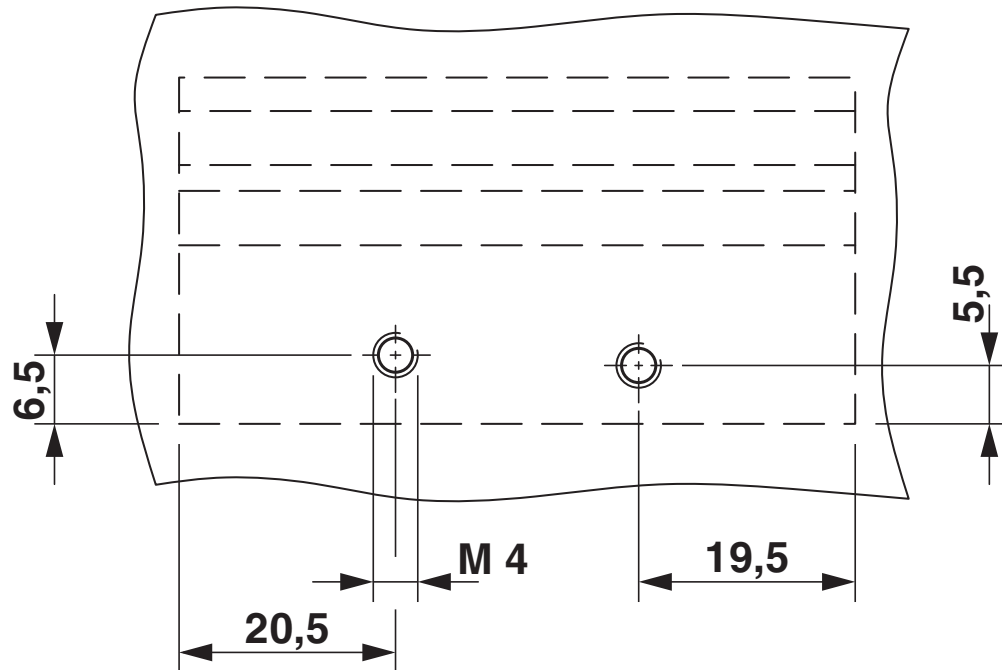
Drilling diagram
