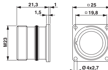
Dimensional drawing
