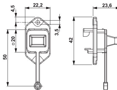
Sealing plug for push-pull panel mounting frame
