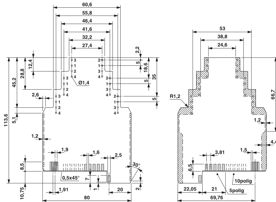
Dimensioned drawing
