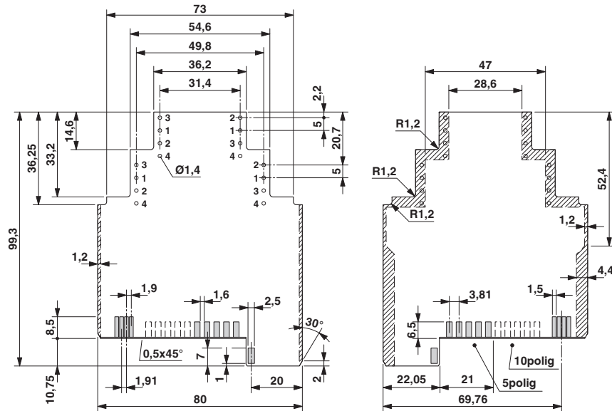
Dimensioned drawing
