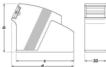
Dimensions: VC-MEMV-T...M...
