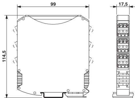
Figure 1 Dimensions
