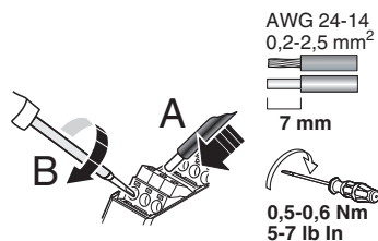
Figure 4 Wire connections
