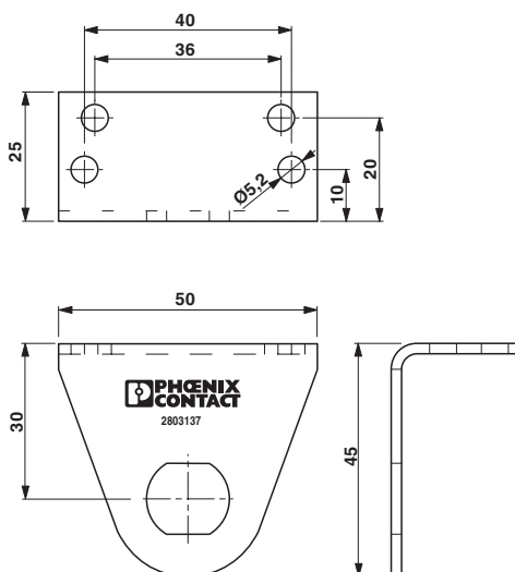
Dimensional drawing
