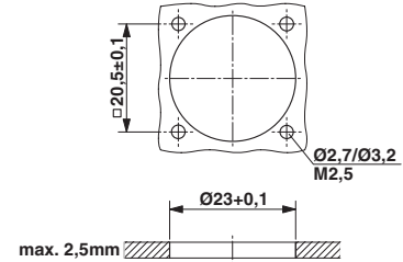
Dimensioned drawing
