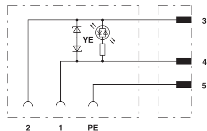
Contact assignment
