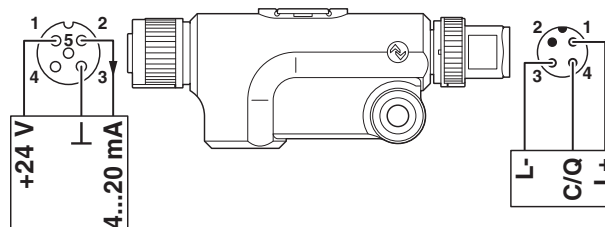
Figure 5 Connection example
