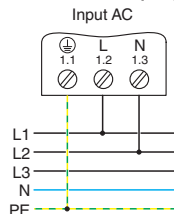
Figure 16 Wiring principle in a star supply system, two-phase operation
