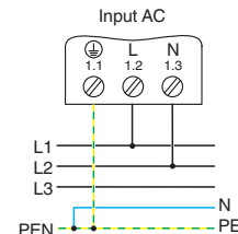
Figure 16 Wiring principle in a star supply system, two-phase operation
