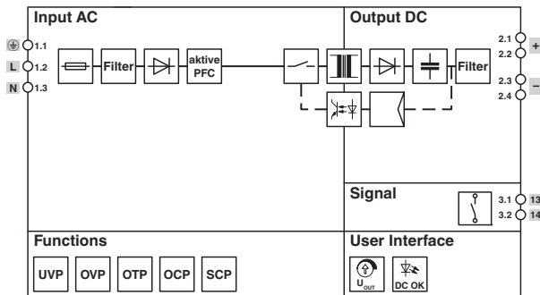
Figure 4 Block diagram
