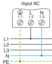
Figure 15 Wiring principle in a star supply system, single-phase operation
