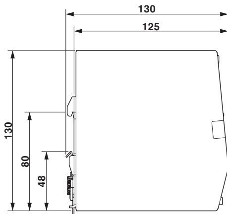
Figure 6 Device dimensions (dimensions in mm)
