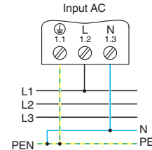
Figure 15 Wiring principle in a star supply system, single-phase operation
