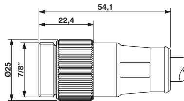
7/8" connector, straight
