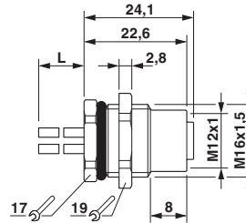
Dimensioned drawing
