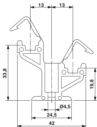
Dimensional drawing
