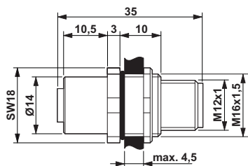
Dimensioned drawing
