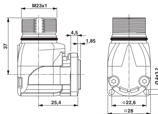
Dimensioned drawing
