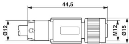
Dimensioned drawing
