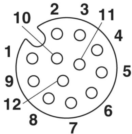
Schematic diagram
