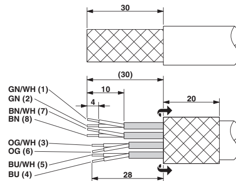
Dimensioned drawing
