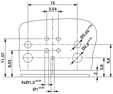
Drilling diagram
