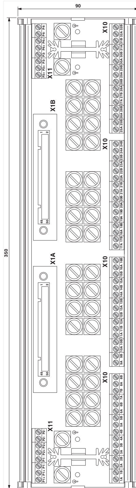
Dimensional drawing
