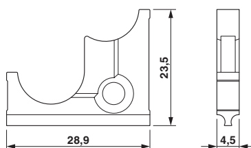
Dimensional drawing
