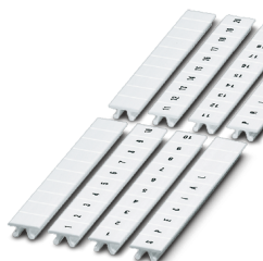
Zack marker strip, 10-section, horizontally labeled with the consecutive numbers: 131 ... 140, white, for terminal block width: 8.2 mm
