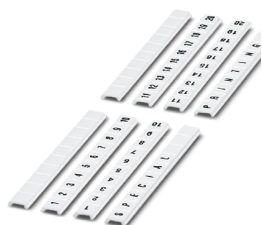
Zack marker strip flat, 10-section, horizontally labeled with the consecutive numbers: 31 ... 40, white, for terminal block width: 6.2 mm
