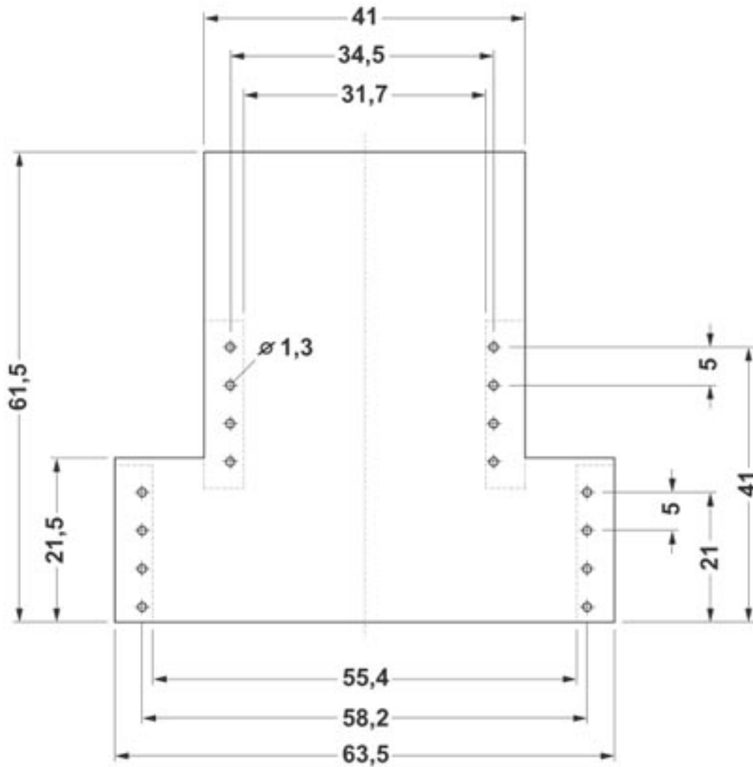
Dimensional drawing of the IEG D-22,5 (4-pos.) PCBs
