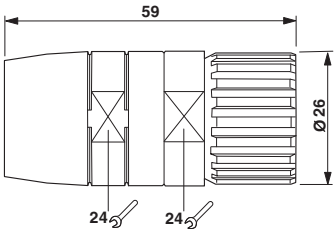
Dimensioned drawing
