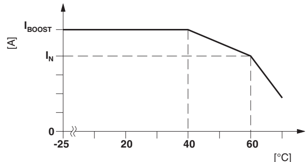
Figure 12 Derating diagram
