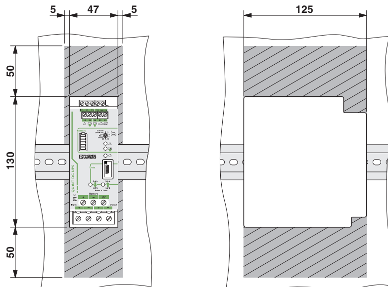
Figure 4 Installation dimensions
