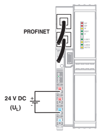
Connection diagram
