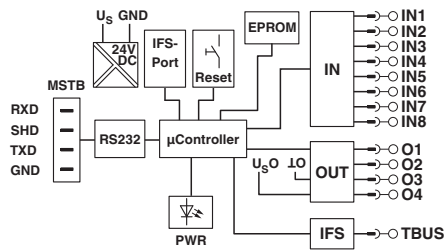
Block diagram
