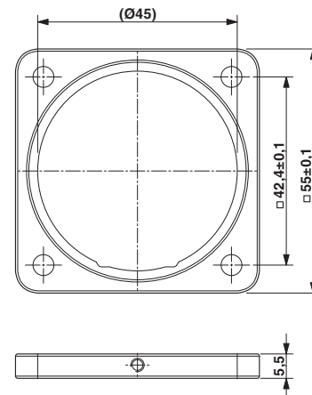
Dimensioned drawing
