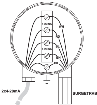
Circuit diagram
