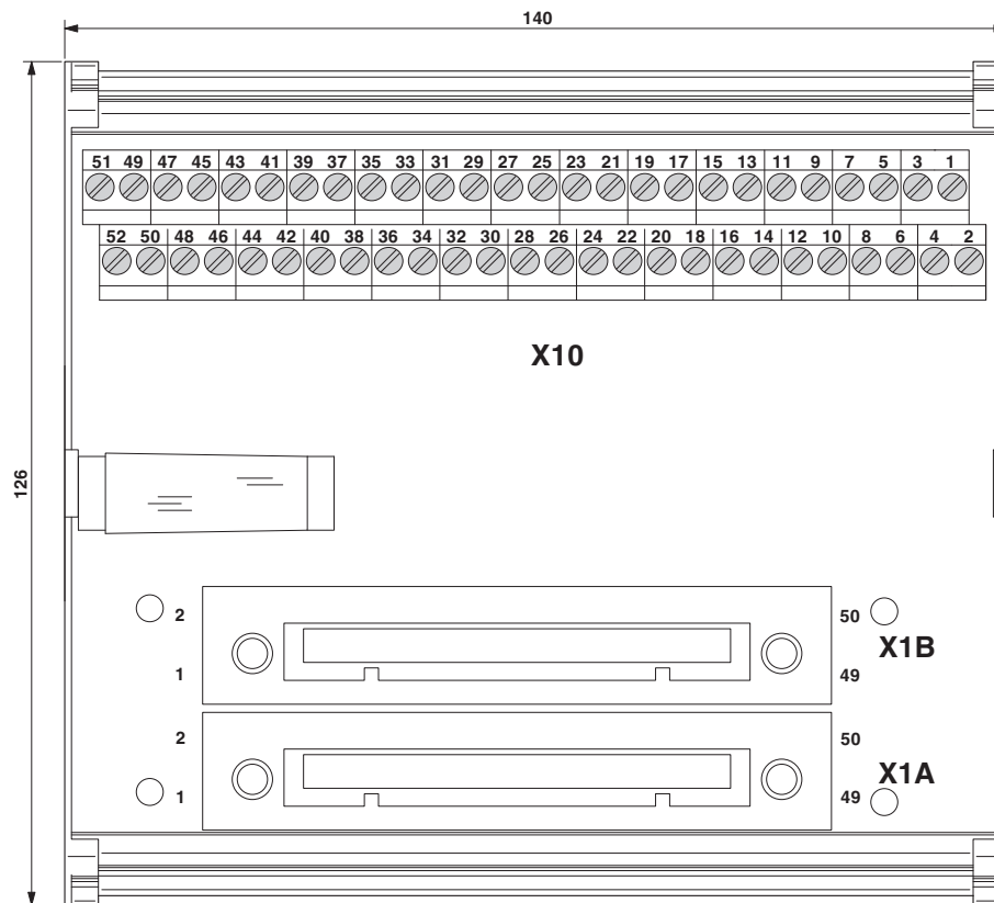
Dimensional drawing
