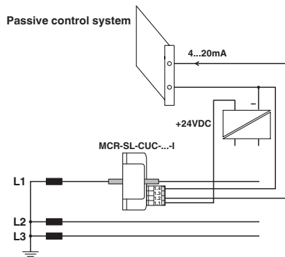
Application drawing
