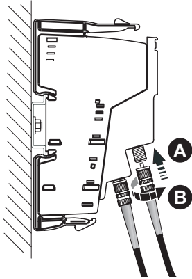
Figure 2 Connecting the remote bus cables
