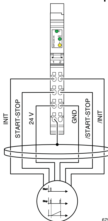
Figure 3 Typical connection
