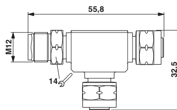
M12 T-distributor
