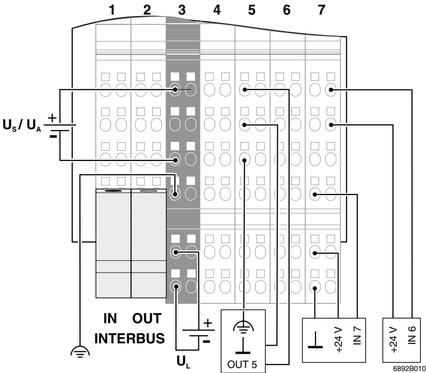
Figure 5 Connection example
