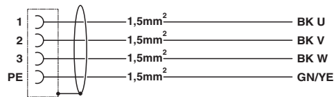
Circuit diagram
