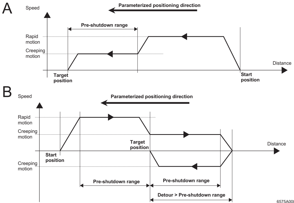
Figure 8 Backlash compensation
