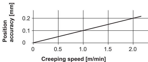
Figure 13 Position accuracy
