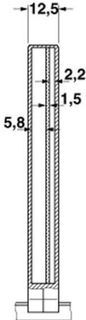
Dimensioned drawing
