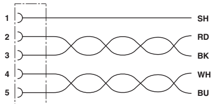
Contact assignment of 7/8"-16UNF socket
