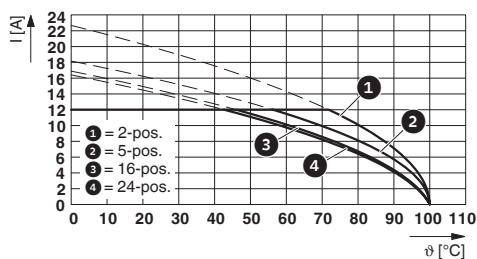
Type: MVSTBW 2,5/...-ST-5,08 with SMSTB 2,5/...-G-5,08
