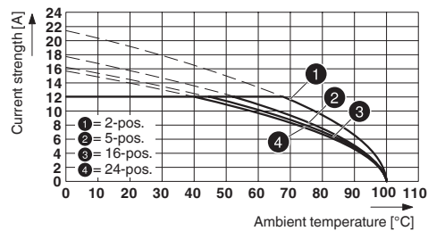
Type: MVSTB(R/W) 2,5/...-ST-5,08 with MSTBW 2,5/...-G-5,08
