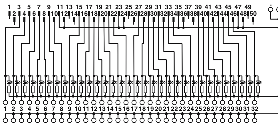
Connection diagram
