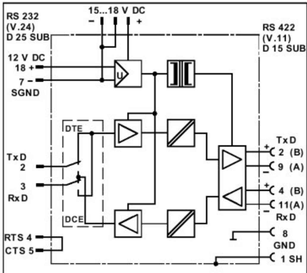
Circuit diagram
