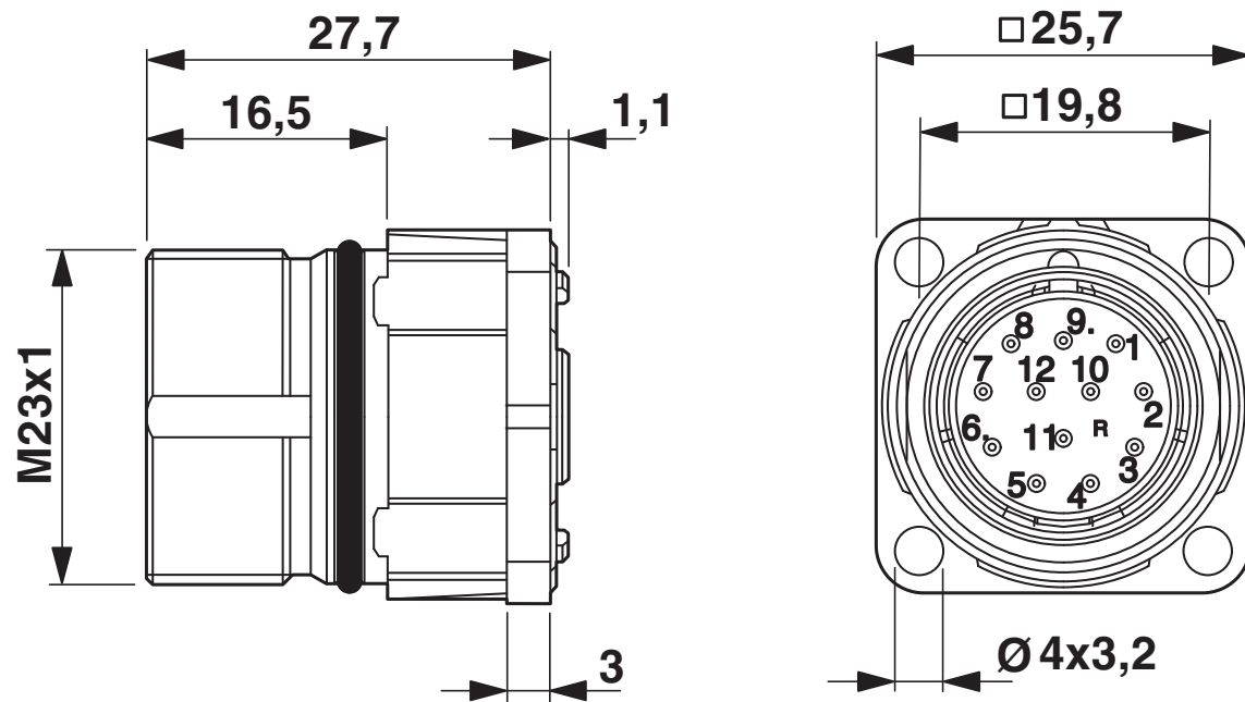
Dimensioned drawing
