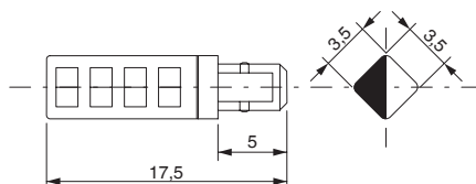
Dimensional drawing
