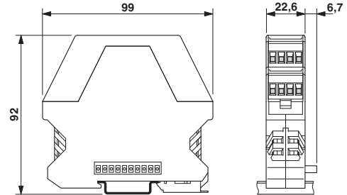
Dimensions of the electronic housing ME 22.5 flat.../BUS 5... and ME 22.5 flat.../BUS 10... with double-level upper part
